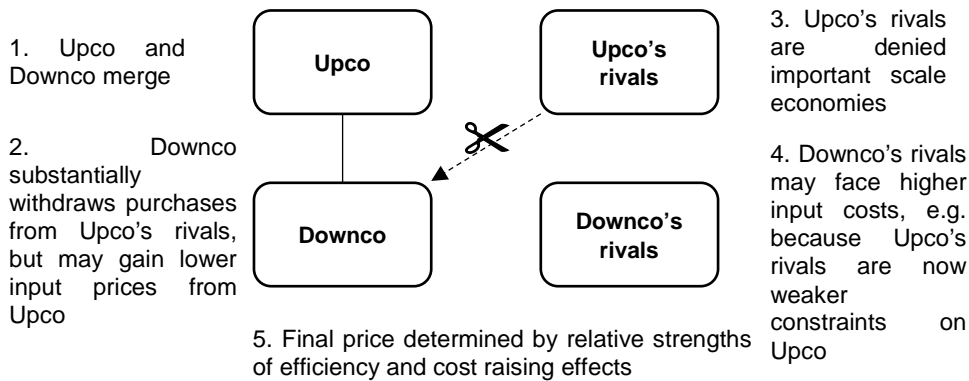
Diagram 2: Customer Foreclosure
