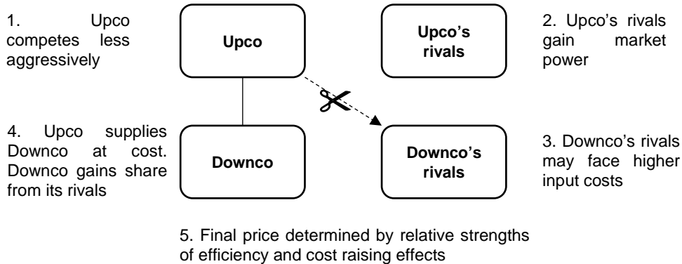
Diagram 1: Input Foreclosure
